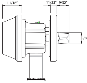
LU - SINGLE CYLINDER (200)
