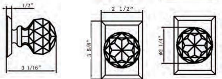
926-1 Shown in US10B Also available in: PVD, US4, US15, US19, US26 Passage/Privacy Dummy
