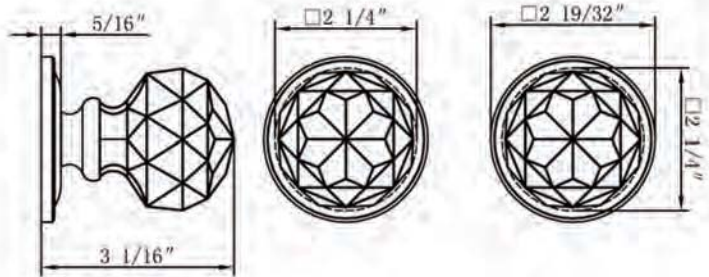
926-0 Shown in US26 Also available in: PVD, US4, US10B, US15, US19 Passage/Privacy Dummy
