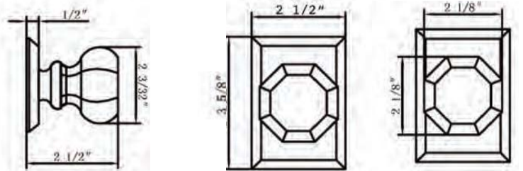
925-1 Shown in US10B Also available in: PVD, US4, US15, US19, US26 Passage/Privacy Dummy
