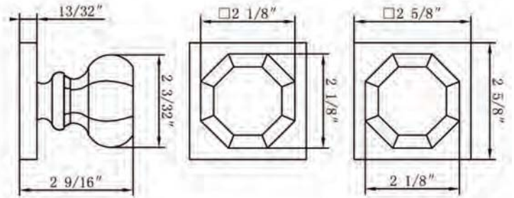
925-7 Shown in US10B Also available in: US4, US15, US19, US26 Passage/Privacy Dummy
