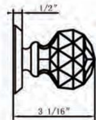
926G-1 Shown in US10B Also available in: PVD, US4, US15, US19, US26 Passage/Privacy Dummy
